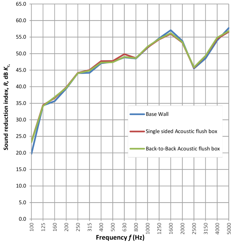
Sound reduction index, R , in accordance with ISO 10140-2
